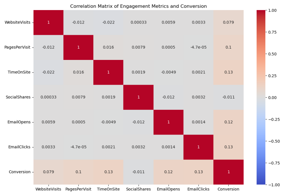
Figure 4 Correlation Matrix
