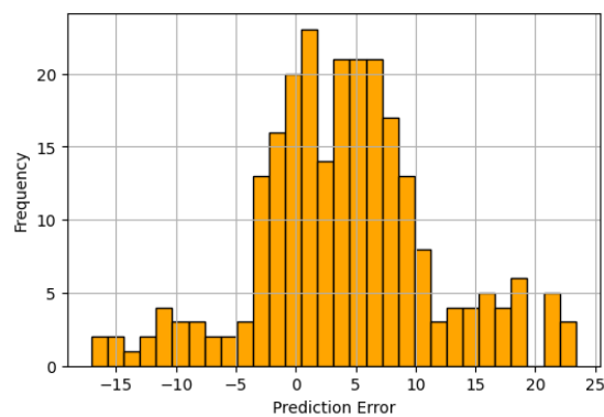
Figure 4 Error distribution histogram for the Hybrid SARIMAX–LSTM model
